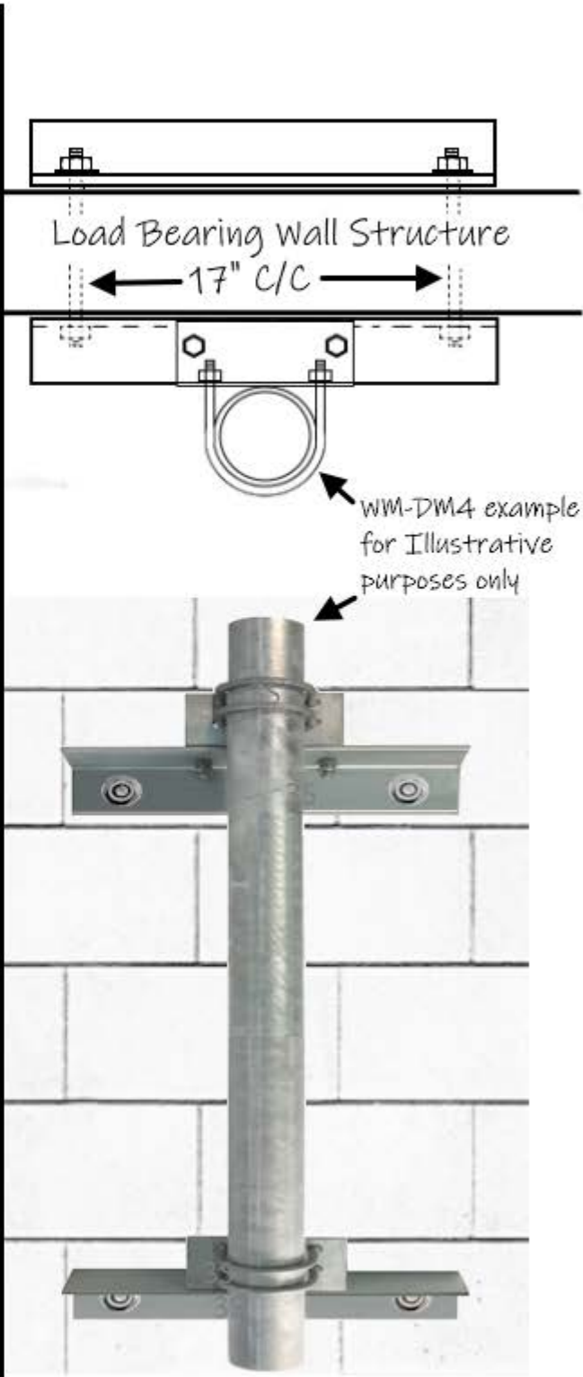
Antenna Mounting Assembly Typical Installation Example
