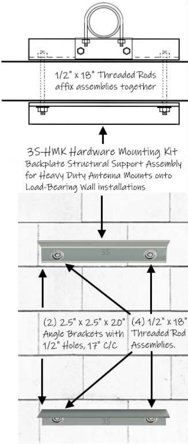
3S-HMK Hardware Mounting Kit Breakout and Illustrative Detail
