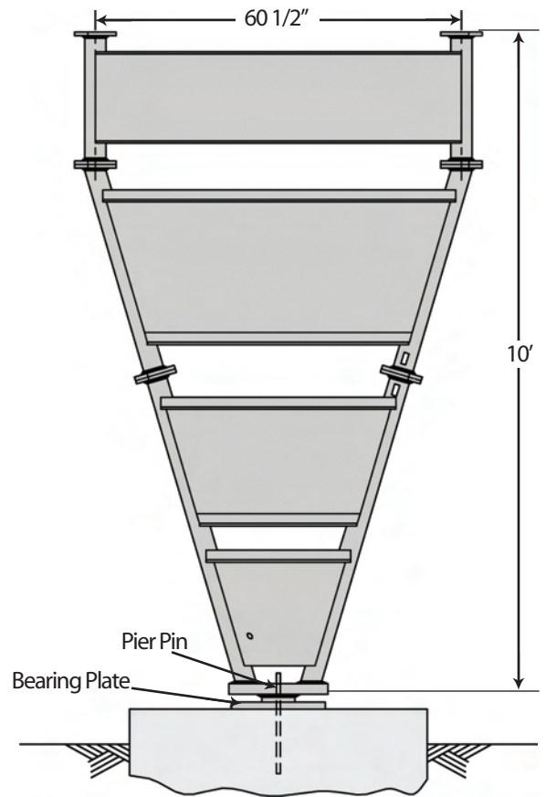
TAPERED BASE
