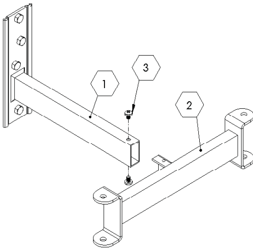
Step 3: Attaching the connector support to the wall plate
