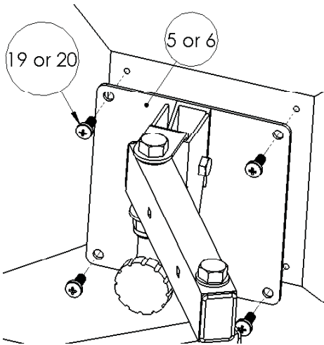
Step 5: Attaching the TVs to the LCD-1s
