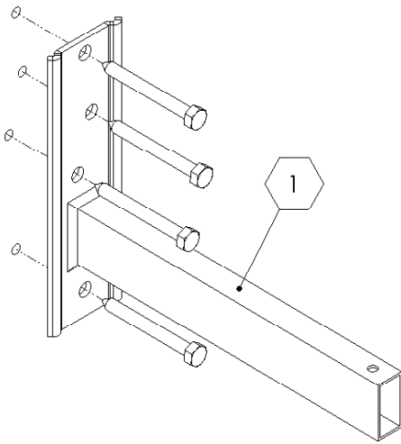
Step 2: Attaching the wall plate to the wall (Lag screws are not included)
