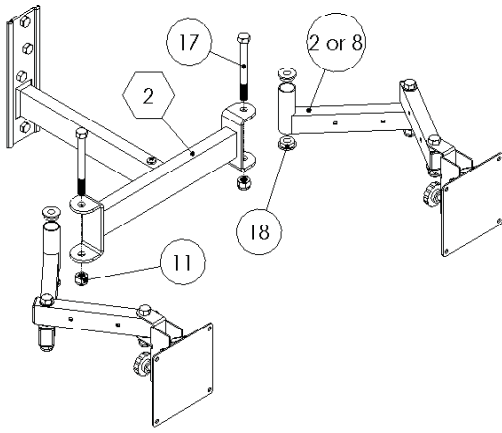
Step 4: Attaching the LCD-1s to the connector support
