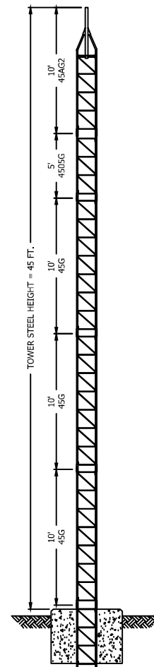
P/N: 45SS045 45' 45G SERIES TOWER ASSEMBLY
