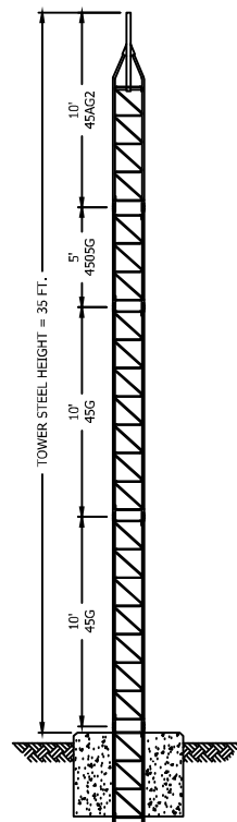
P/N: 45SS035 35' 45G SERIES TOWER ASSEMBLY
