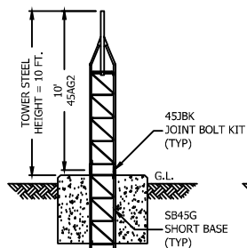
P/N: 45SS010 10' 45G SERIES TOWER ASSEMBLY
