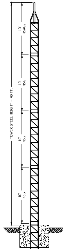
P/N: 45SS040 40' 45G SERIES TOWER ASSEMBLY
