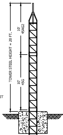
P/N: 45SS020 20' 45G SERIES TOWER ASSEMBLY
