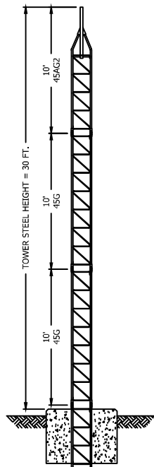
P/N: 45SS030 30' 45G SERIES TOWER ASSEMBLY
