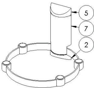
Step 4: Connecting the support ring to the wall plate
